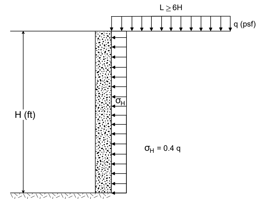
E) Lateral Pressure Due to Uniform Surcharge. (For L \leq 6H Use Chart D Above)
